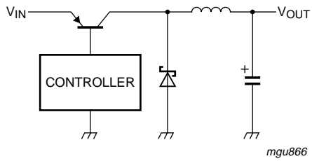
Fig 9. DC-to-DC converter.
