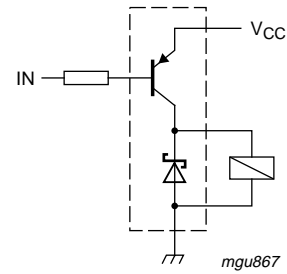
Fig 10. Inductive load driver (relays, motors and buzzers) with free-wheeling diode.
